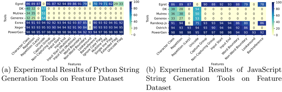
Fig. 3. Experimental Results of String Generation Tools on Feature Dataset
